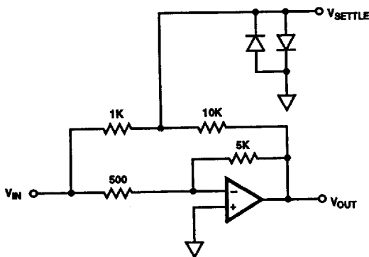
FIGURE 3. SETTLING TIME SCHEMATIC
