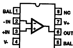
HFA-0002 (PDIP, CDIP, SOIC) TOP VIEW
