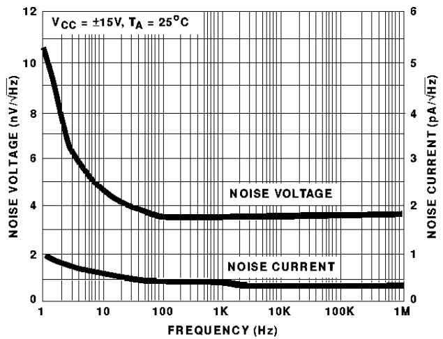
FIGURE 6. NOISE CHARACTERISTICS
