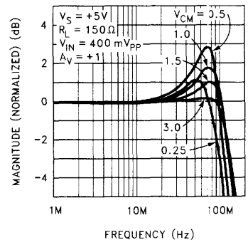
Non-Inverting Frequency Response vs Common Mode Voltage
