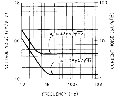
Voltage and Current Noise vs Frequency
