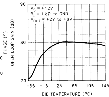
Open Loop Voltage Gain vs Die Temperature
