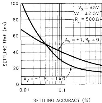
Settling Time vs Settling Accuracy
