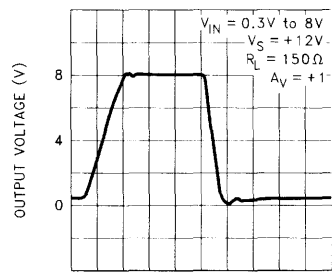
Large Signal Step Response, V_S = +12V
