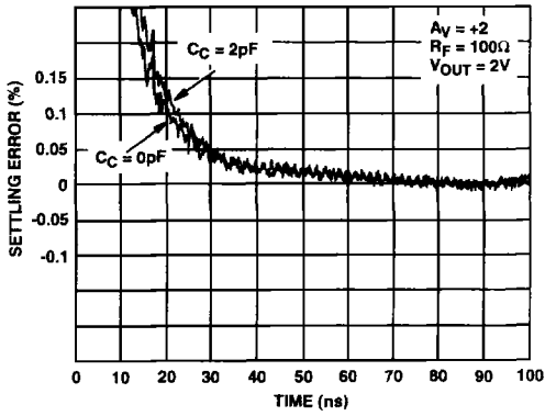
FIGURE 41. SETTling RESPONSE
