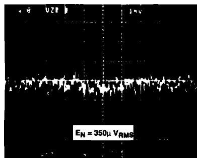
FIGURE 2. HFA1106 NOISE PERFORMANCE, UNCOMPENSATED, A_V = +2 , R_F = 100\Omega
