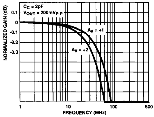
FIGURE 24. GAIN FLATNESS
