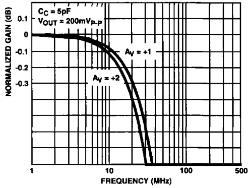
FIGURE 36. GAIN FLATNESS
