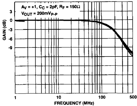
FIGURE 25. FREQUENCY RESPONSE (12 UNITS, 4 RUNS)
