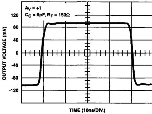
FIGURE 5. SMALL SIGNAL PULSE RESPONSE
