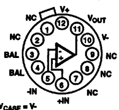
HA2-2541 (TO-8 CAN) TOP VIEW
