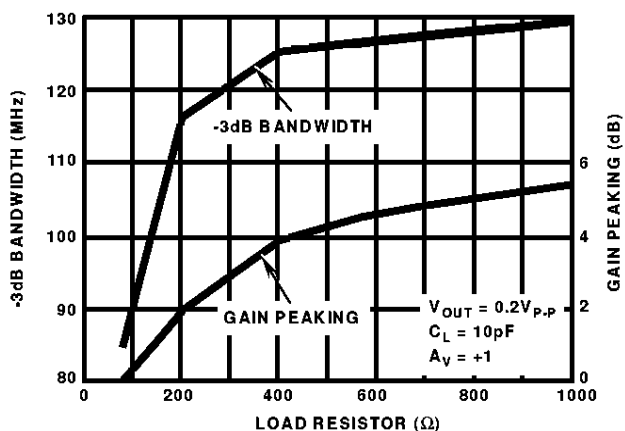
FIGURE 6. BANDWIDTH AND GAIN PEAKING vs LOAD RESISTANCE
