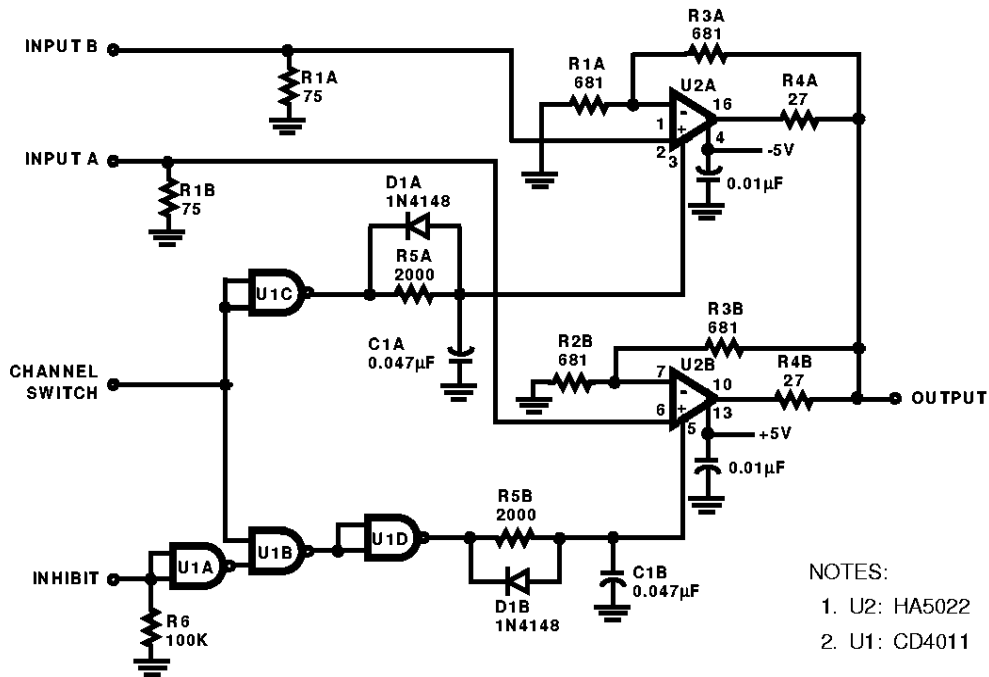
FIGURE 40. LOW IMPEDANCE MULTIPLEXER
