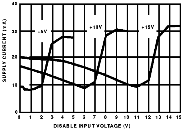
FIGURE 25. SUPPLY CURRENT vs DISABLE INPUT VOLTAGE
