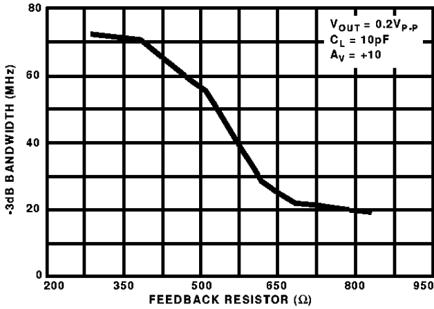
FIGURE 7. BANDWIDTH vs FEEDBACK RESISTANCE
