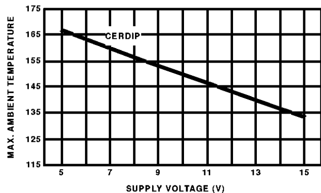
FIGURE 37. MAXIMUM OPERATING AMBIENT TEMPERATURE vs SUPPLY VOLTAGE
