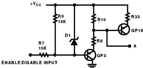
FIGURE 38. SIMPLIFIED SCHEMATIC OF ENABLE/DISABLE FUNCTION
