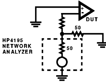
FIGURE 2. TEST CIRCUIT FOR TRANSMITTANCE MEASUREMENTS
