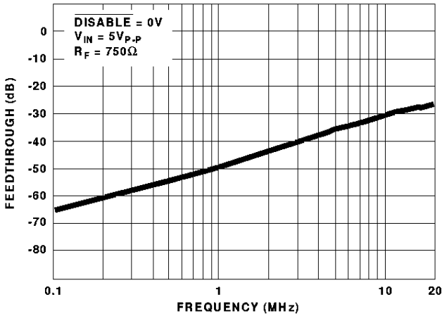
FIGURE 33. DISABLE FEEDTHROUGH vs FREQUENCY
