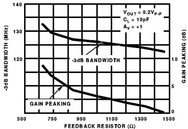
FIGURE 4. BANDWIDTH AND GAIN PEAKING vs FEEDBACK RESISTANCE
