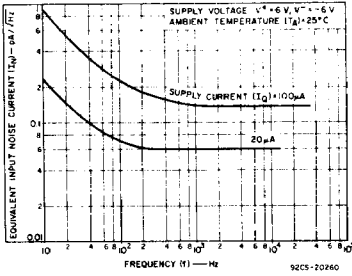
Fig.3— I_N vs. Frequency for CA6078A.
