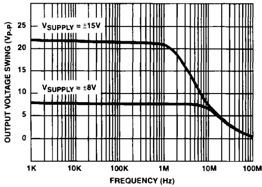
FIGURE 15. MAXIMUM UNDISTORTED OUTPUT SWING vs FREQUENCY
