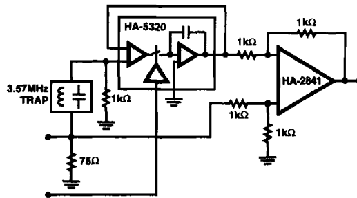
FIGURE 2. VIDEO DC RESTORER
