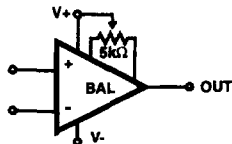
SUGGESTED OFFSET VOLTAGE ADJUSTMENT
