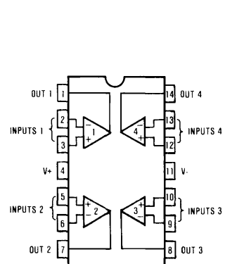
HA1-5144 (CERAMIC DIP) HA3-5144 (PLASTIC DIP)
