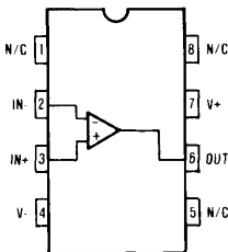
HA1-5141 (CERAMIC MINI-DIP) HA3-5141 (PLASTIC MINI-DIP)
