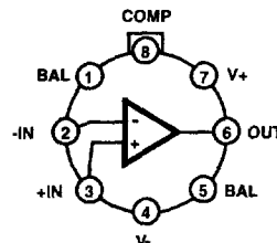
HA-2620, HA-2622, HA-2625 (METAL CAN) TOP VIEW
