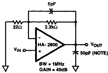
FIGURE 3. VIDEO AMPLIFIER
