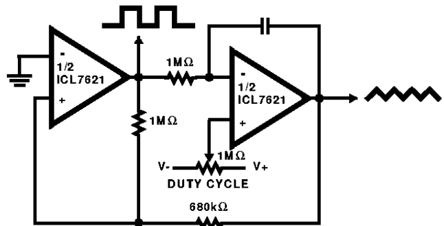
WAVEFORM GENERATOR
