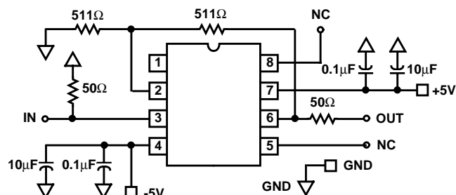
FIGURE 2. HFA11XXEVAL SCHEMATIC
