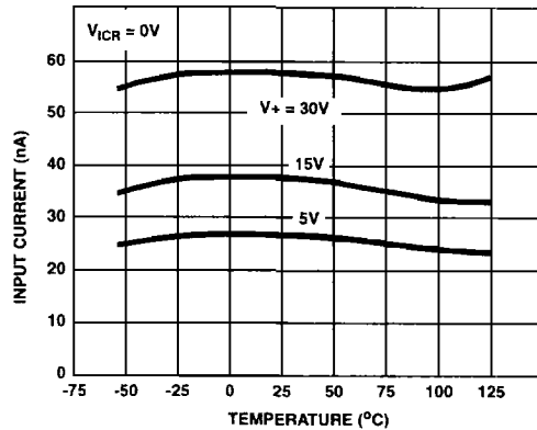
FIGURE 2. INPUT CURRENT vs AMBIENT TEMPERATURE
