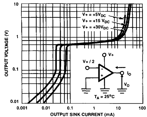
FIGURE 12. OUTPUT SINK CURRENT CHARACTERISTICS
