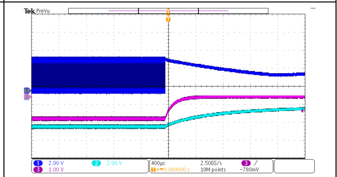
Figure 6. Enable Off Line1: CP, Line2: Vout1, Line3: Vout2
