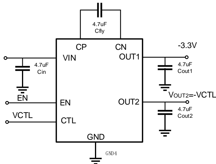
Figure 1. Typical Operation Circuit
