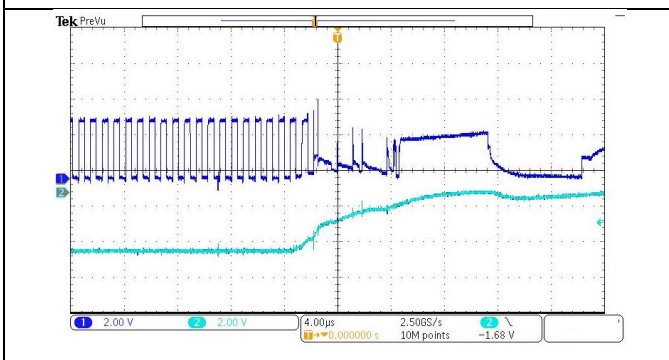
Figure 7. Vout1 short to GND Line1: CP, Line2: Vout1
