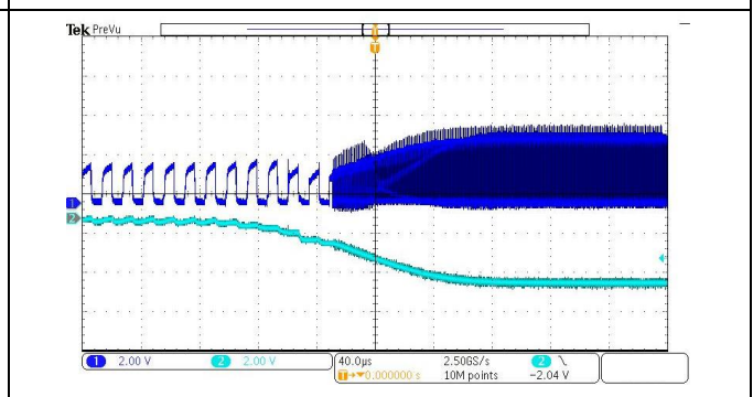
Figure 8. Vout1 Recovery from Short Line1: CP, Line2: Vout1
