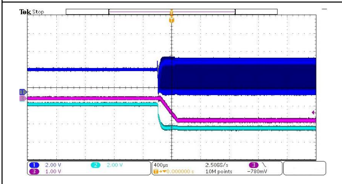
Figure 5. Enable ON Line1: CP, Line2: Vout1, Line3: Vout2
