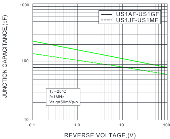
FIG.5-TYPICAL JUNCTION CAPACITANCE
