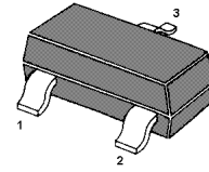
Marking Code: FD TO-236 Plastic Package
