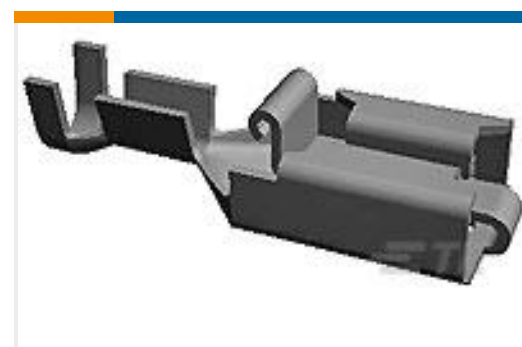
TE Part #1-160759-2 250 PL MKI REC. 20-15AWG PTPB
