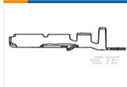
TE Part #172775-1 MIC MK-2 REC B TYPE
