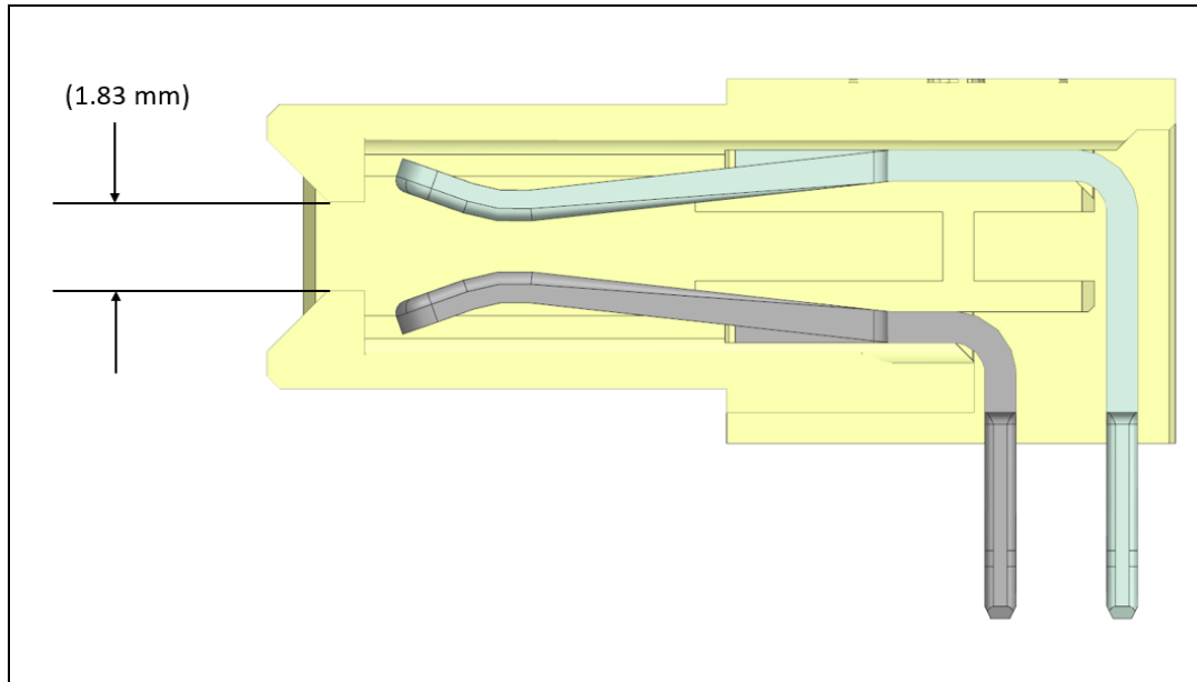
Hybrid Right-Angle Receptacle
