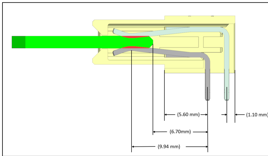
Edge Card mated with Hybrid Right-Angle Receptacle
