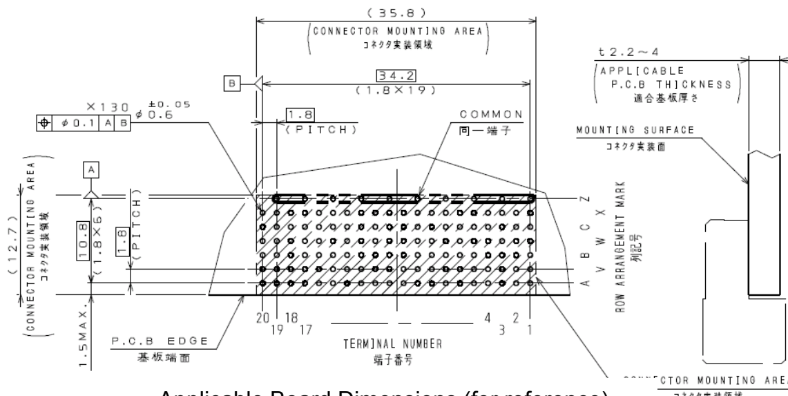
Applicable Board Dimensions (for reference)
