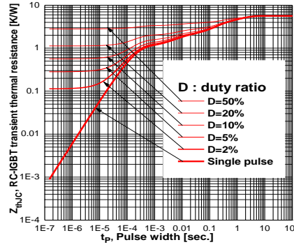
IGBT transient thermal resistance at all six IGBTs operation
