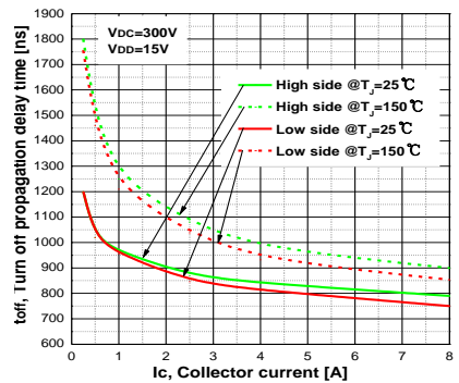
Typ. Turn off propagation delay time
