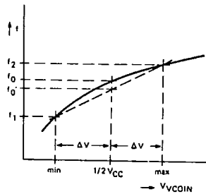
Fig. 35 - Definition of VCO frequency linearity.
