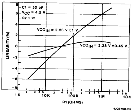
Fig. 36 - HC7046A VCO linearity vs. R1.
