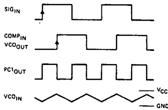
Fig. 3 - Typical waveforms for PLL using phase comparator 1, loop locked at f_0 .
