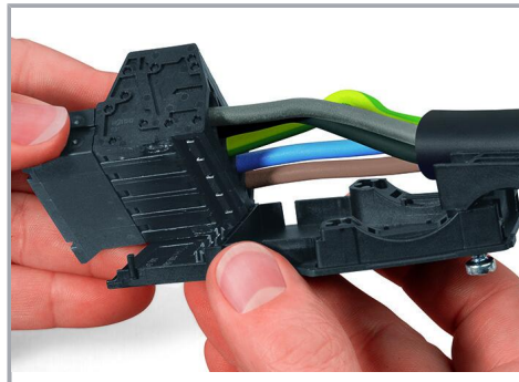
Snap wired connector onto the base.
