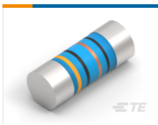
TE Part #7-2176314-8 MELF SMA-A 56R 1% 50PPM 0102 0.3 W
