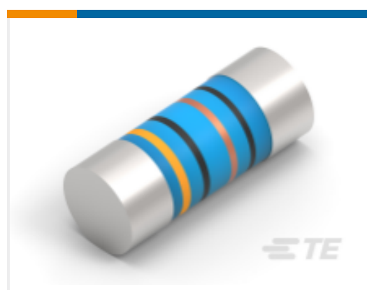
TE Part #4-2176314-1 MELF SMA_A 330R 1% 50PPM 0102 0.3 W
