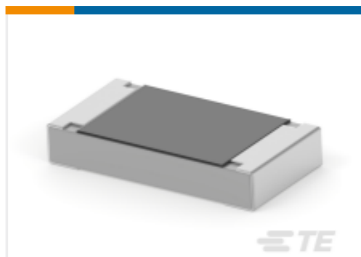
TE Part #1-2176344-8 CRGCQ 1206 680R 5%
