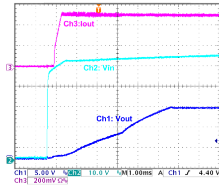
上电 (HT7463B, V IN =52V, I OUT =500mA)
