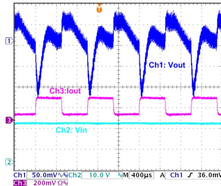
负载瞬变 (HT7463B, I OUT =50mA~200mA)
