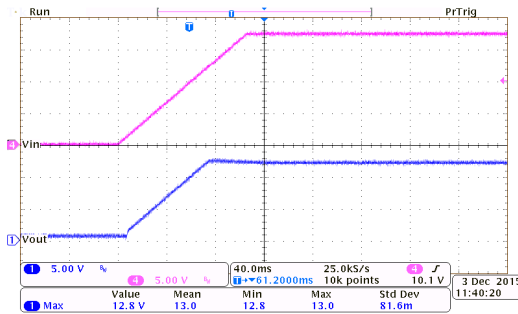
上电响应: HT75C0-7 ( I_{OUT}=0mA , T_{RISE}=100ms )
