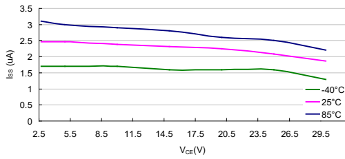
I SS vs V CE : HT7533-7 (I OUT =0mA)
