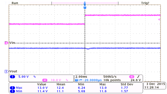
线性瞬态响应: HT75C0-7 ( I_{OUT}=10mA )
