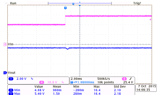
线性瞬态响应: HT7550-7 ( I_{OUT}=10mA )
