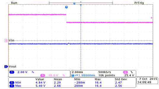
线性瞬态响应: HT7550-7 ( I_{OUT}=10mA )
