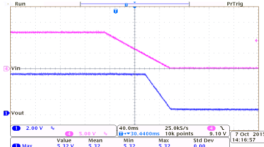
掉电响应: HT7550-7 ( I_{OUT}=0mA , T_{FALL}=100ms )
