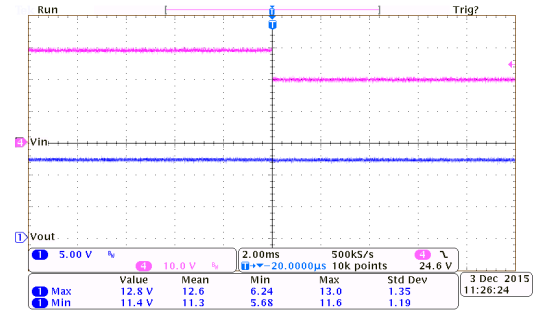
线性瞬态响应: HT75C0-7 ( I_{OUT}=10mA )
