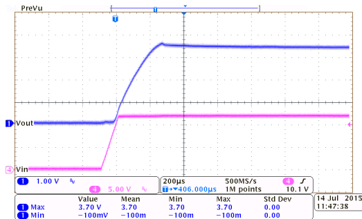
上电响应：HT7333-2 ( I_{OUT}=0mA , T_{RISE}=0.1ms )
