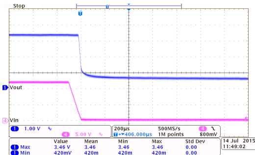
HT7333-2 ( I_{OUT}=0mA , T_{FALL}=0.1ms )
