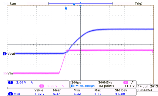
HT7350-2 ( I_{OUT}=250mA , T_{RISE}=0.1ms )
