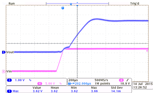
HT7333-2 ( I_{OUT}=250mA , T_{RISE}=0.1ms )
