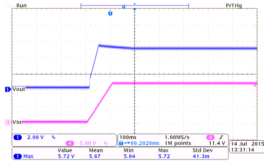
HT7350-2 ( I_{OUT}=0mA , T_{RISE}=100ms )
