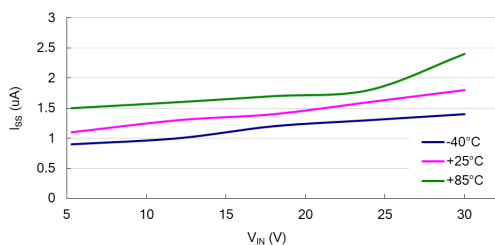
I_{SS} vs V_{IN} : HT7333-2 ( I_{OUT}=0mA )
