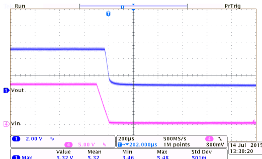
HT7350-2 ( I_{OUT}=0mA , T_{FALL}=0.1ms )
