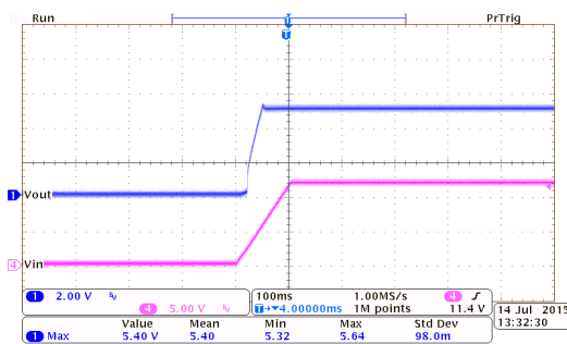
HT7350-2 ( I_{OUT}=250mA , T_{RISE}=100ms )
