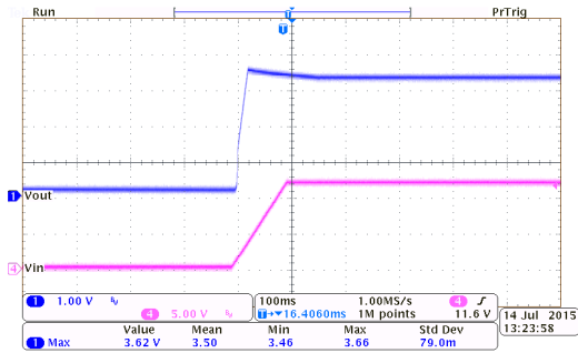
HT7333-2 ( I_{OUT}=0mA , T_{RISE}=100ms )
