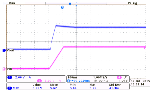
HT7350-1 ( I_{OUT}=0mA , T_{RISE}=100ms )
