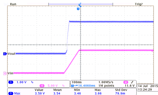
HT7333-1 ( I_{OUT}=250mA , T_{RISE}=100ms )
