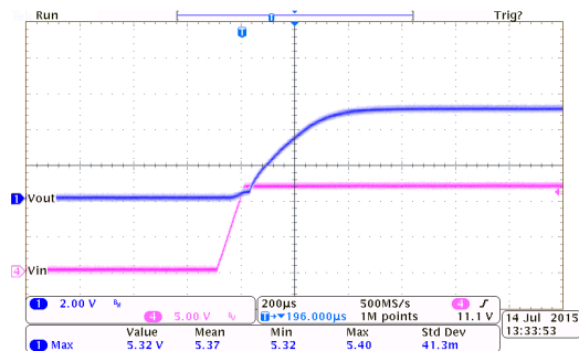
HT7350-1 ( I_{OUT}=250mA , T_{RISE}=0.1ms )
