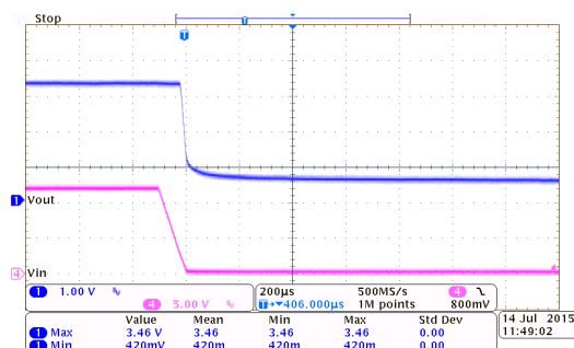
HT7333-1 ( I_{OUT}=0mA , T_{FALL}=0.1ms )
