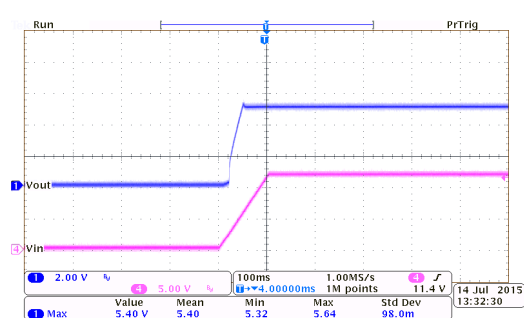
HT7350-1 ( I_{OUT}=250mA , T_{RISE}=100ms )
