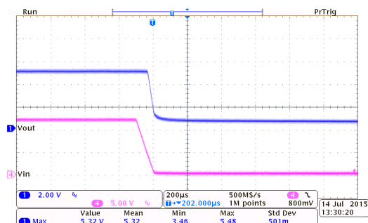
HT7350-1 ( I_{OUT}=0mA , T_{FALL}=0.1ms )
