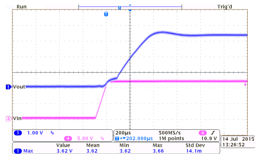
HT7333-1 ( I_{OUT}=250mA , T_{RISE}=0.1ms )
