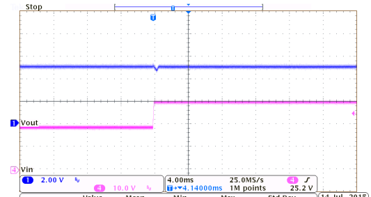
线性瞬态响应: HT7350-1 ( I_{OUT}=10mA )
