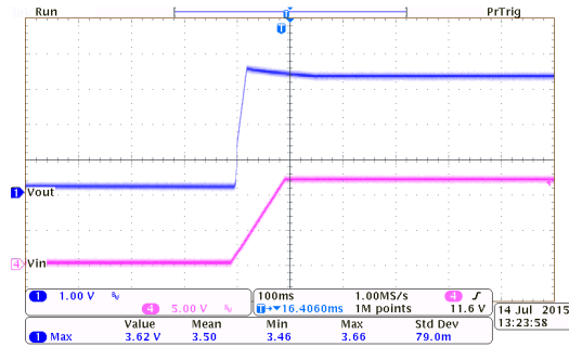
HT7333-1 ( I_{OUT}=0mA , T_{RISE}=100ms )
