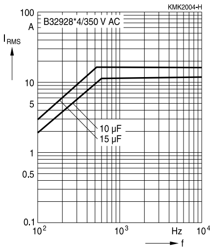
Lead spacing 52.5 mm
