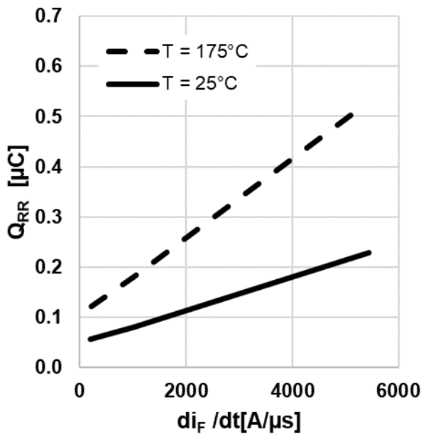
Figure 19 Typical reverse recovery charge as a function of diode current slope ( Q_{rr} = f(di_f/dt) , V_{DD} = 800V , V_{GS} = 0V/15V , I_D = 13A , ind. load, test circuit in Fig.E, body diode at V_{GS} = 0V )
