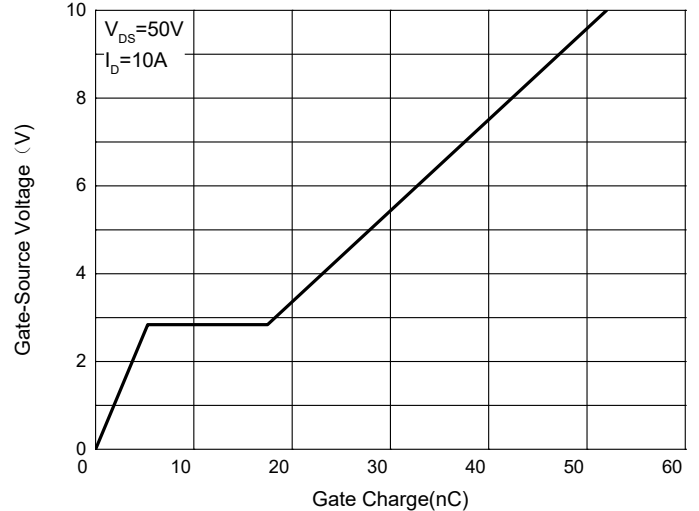
Fig. 6 - Gate Charge
