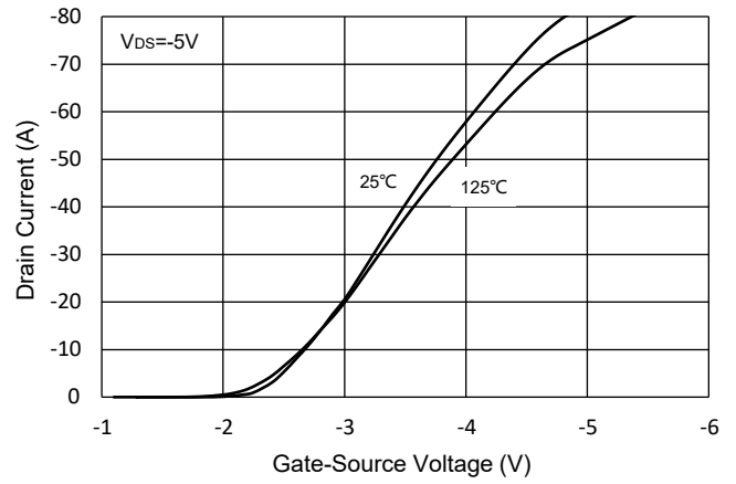
Fig.2 Transfer Characteristic
