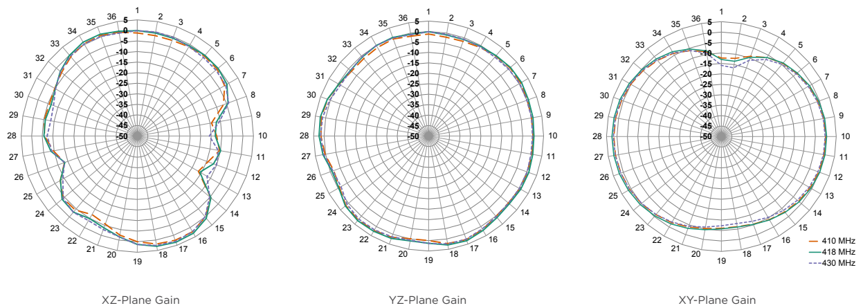
Figure 8. Radiation Patterns for PW 410 MHz Antenna
