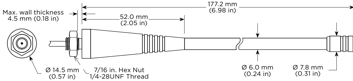
Figure 6. PW 410 MHz Antenna Dimensions
