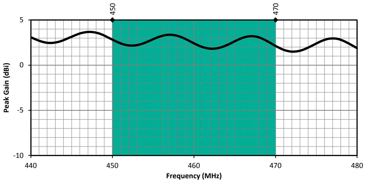
Figure 3. CW 450 MHz Antenna Peak Gain with Band Highlight
