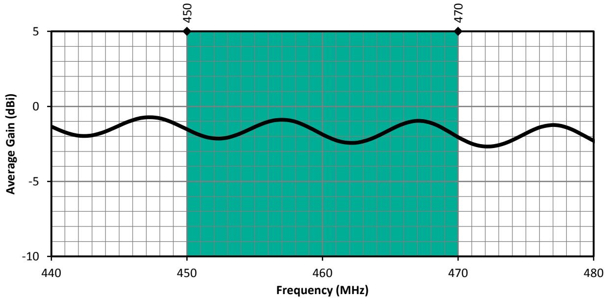
Figure 4. CW 450 MHz Antenna Average Gain with Band Highlight
