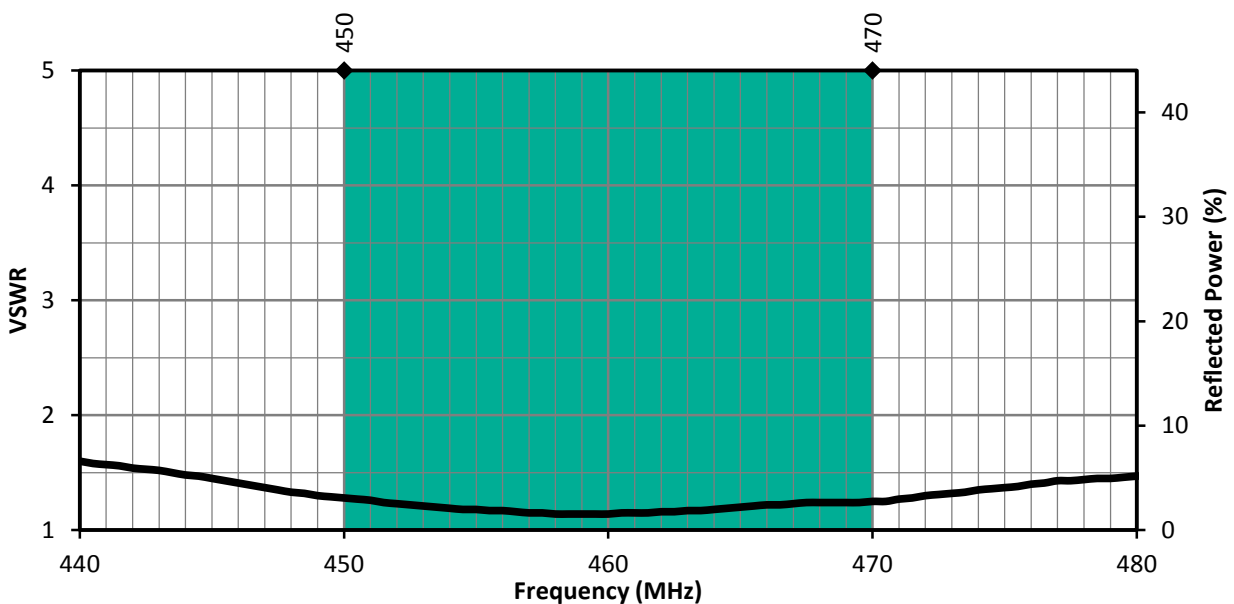
Figure 1. CW 450 MHz Antenna VSWR with Band Highlight
