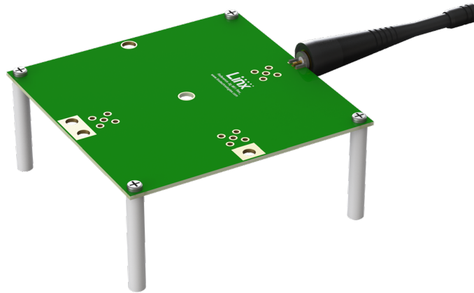
Figure 7. CW 450 MHz Antenna Shown On Edge of Evaluation Board
