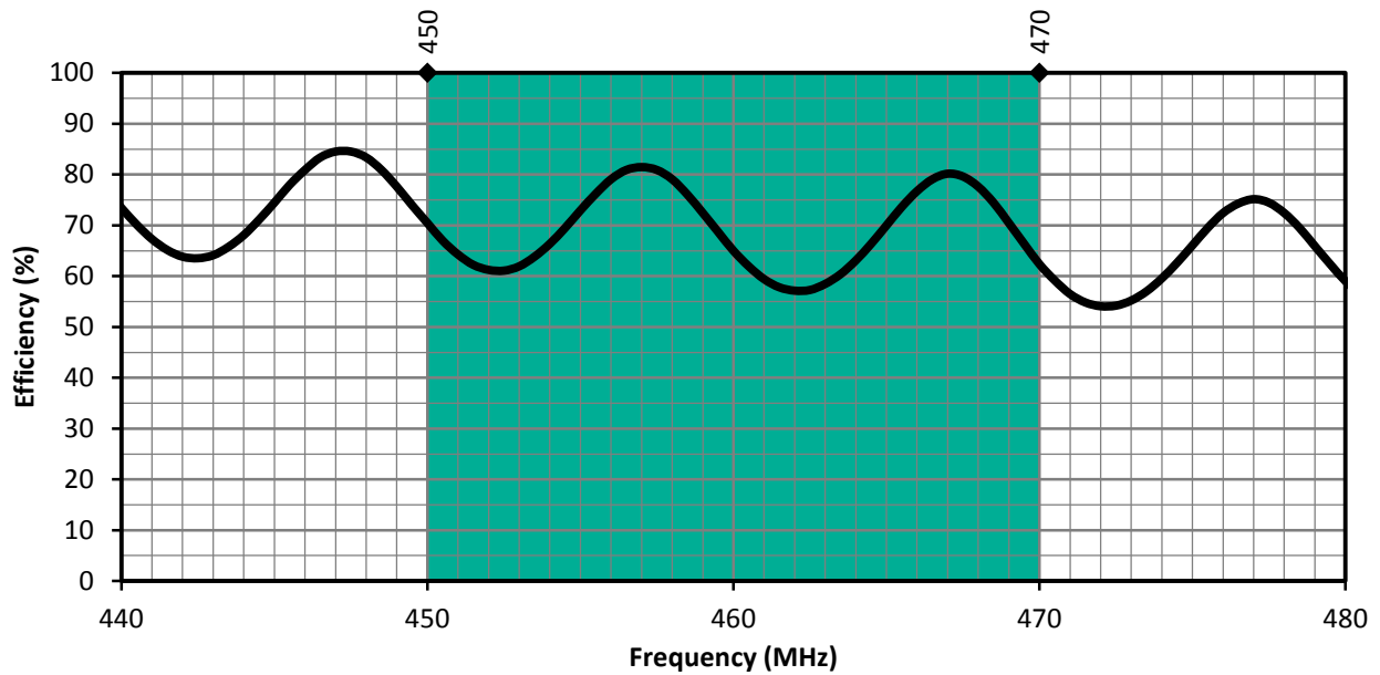
Figure 5. CW 450 MHz Antenna Radiation Efficiency with Band Highlight
