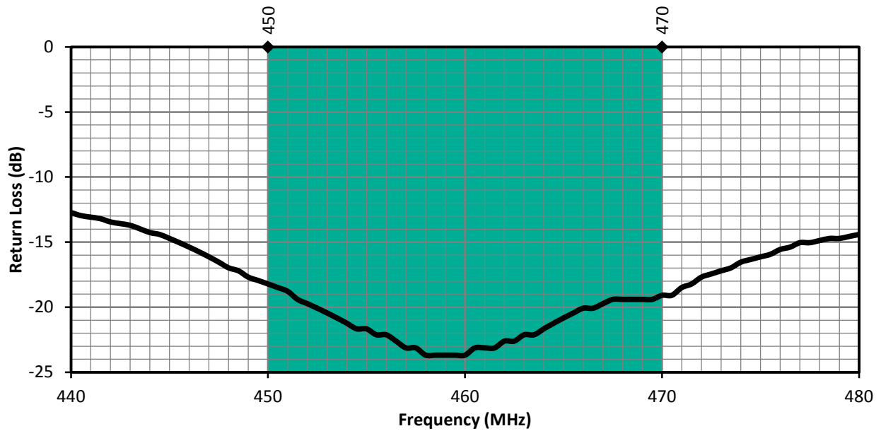
Figure 2. CW 450 MHz Antenna Return Loss with Band Highlight
