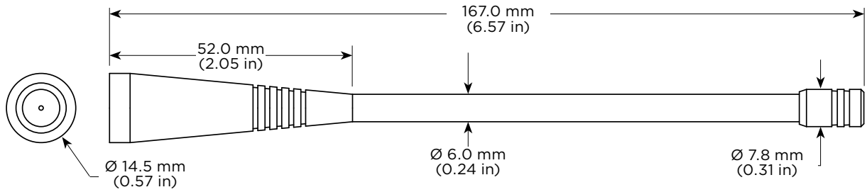
Figure 6. CW 450 MHz Antenna Dimensions
