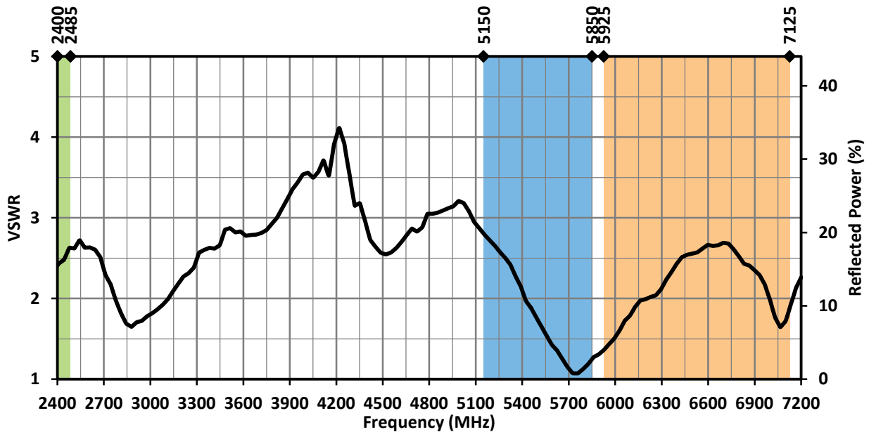
Figure 11. ANT-W63-MON VSWR, Straight
