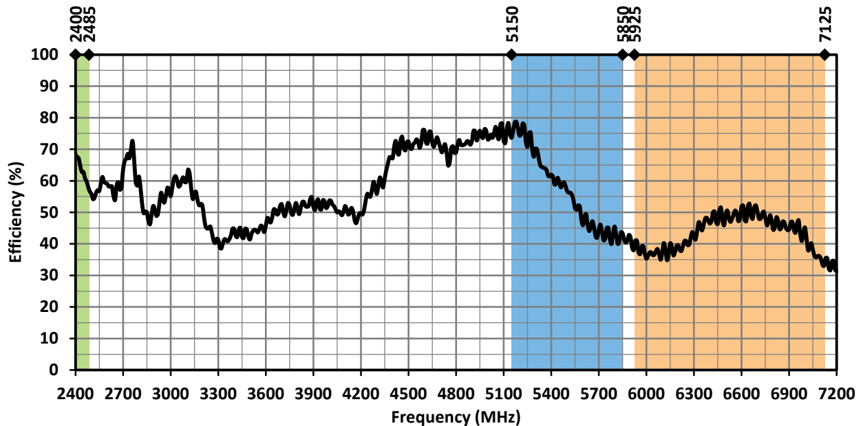
Figure 15. ANT-W63-MON Antenna Efficiency, Straight
