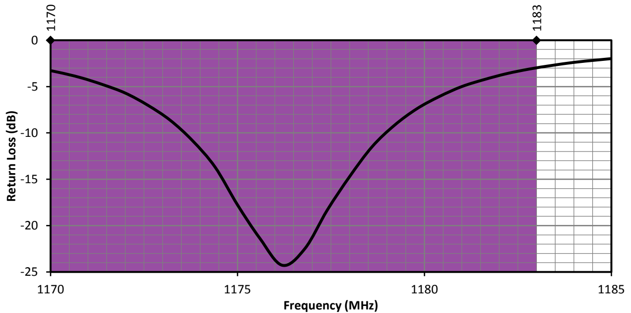
Figure 5. ANT-GNCP-TH258L15 Return Loss, L5 Band
