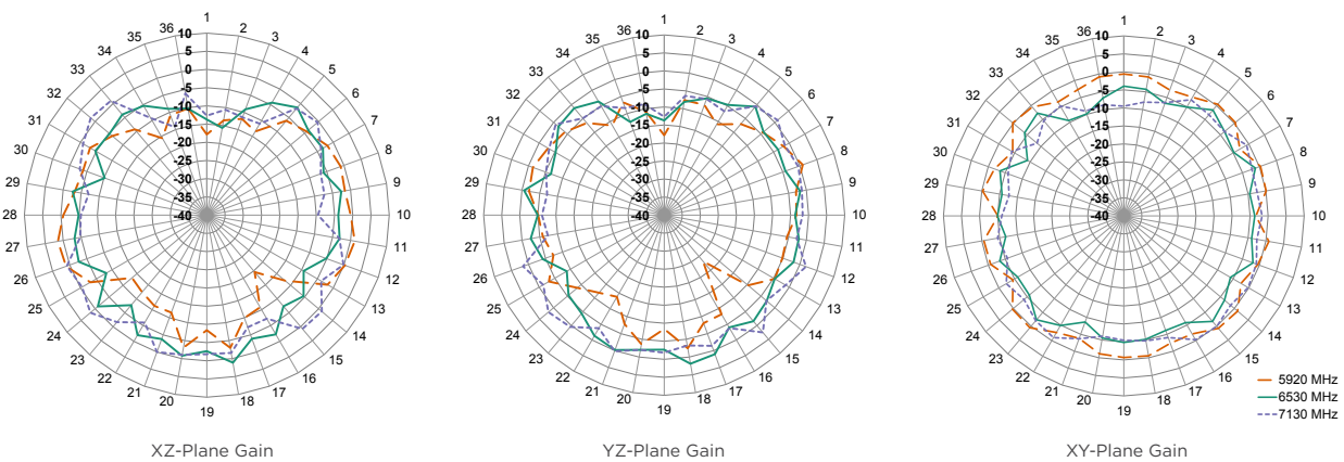
Figure 17. Radiation Patterns for the ANT-W63-WRT Series Antenna at Center of Ground Plane
