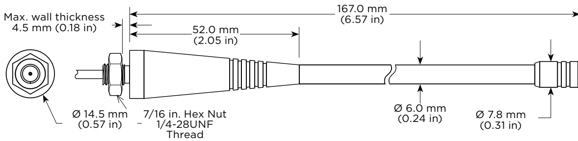
Figure 6. PW 450 MHz Antenna Dimensions
