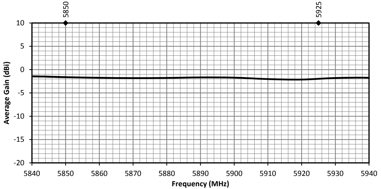
Figure 7. ANT-V2X-IPW1-NP Antenna Average Gain, Free Space
