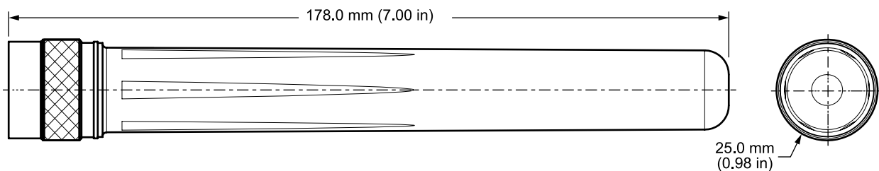
Figure 1. ANT-GNRM-L125A Series Antenna Dimensions
