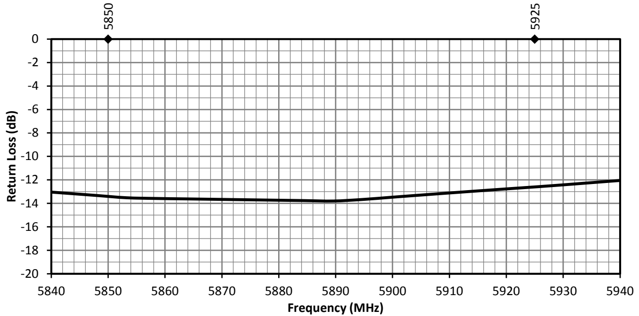
Figure 5. ANT-V2X-IPW1-NP Antenna Return Loss, Free Space
