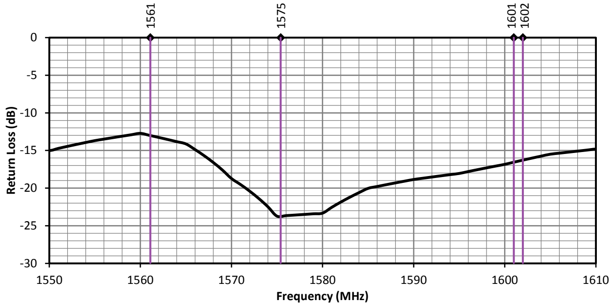
Figure 4. ANT-GNCP-C25L12100 Return Loss, L1 Band
