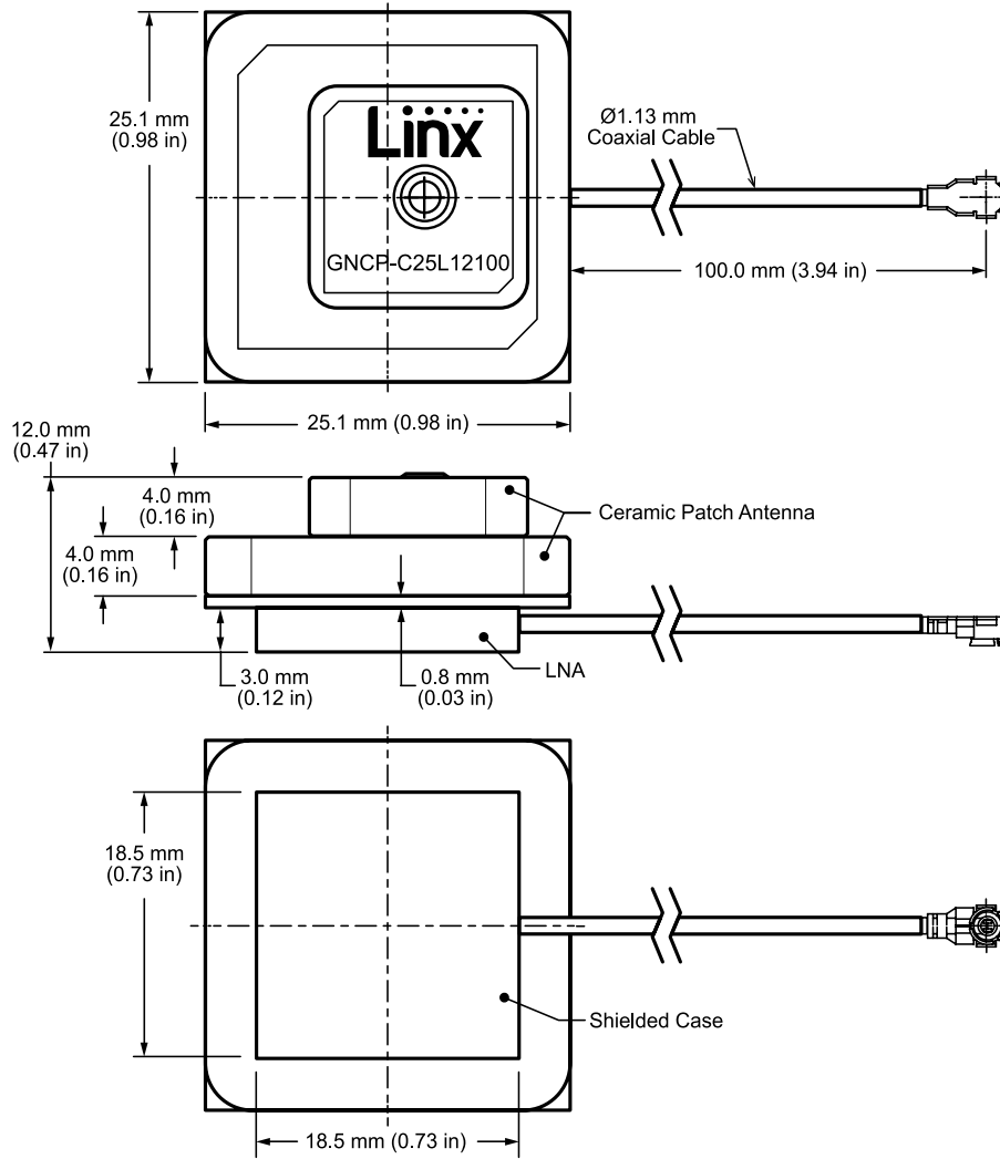
Figure 1. ANT-GNCP-C25L12100 Antenna Dimensions
