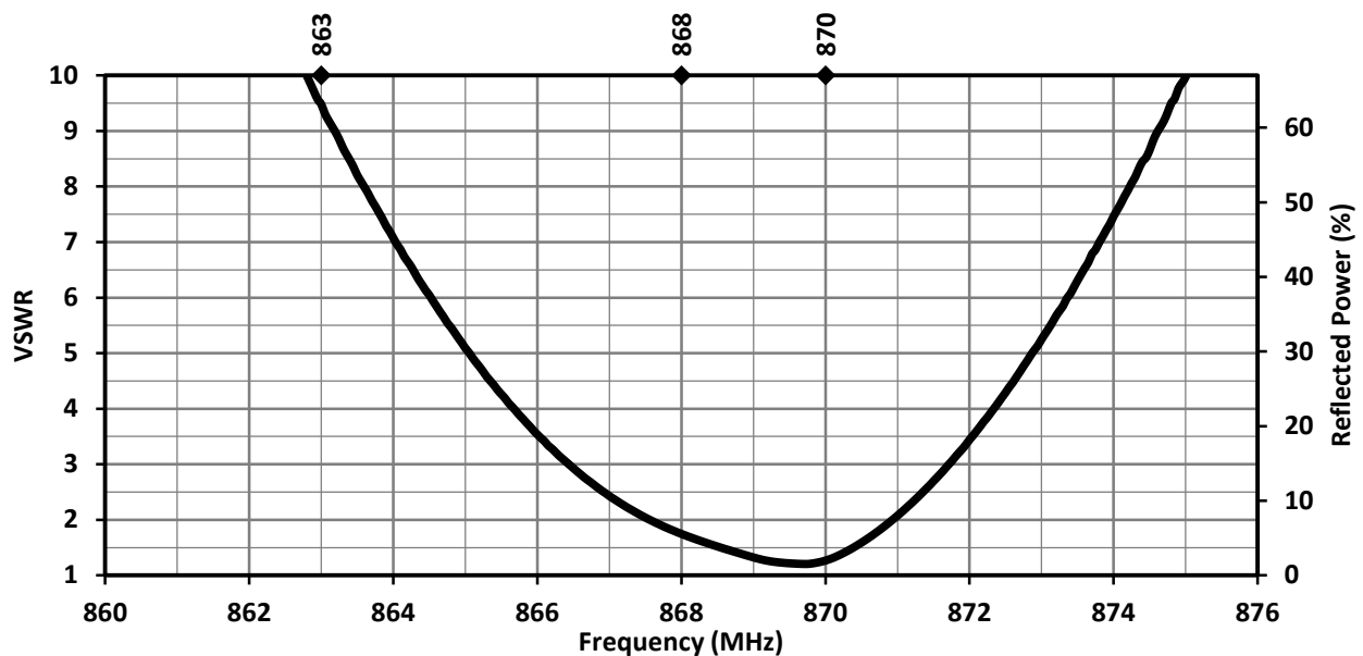
Figure 2. 868-CPA VSWR
