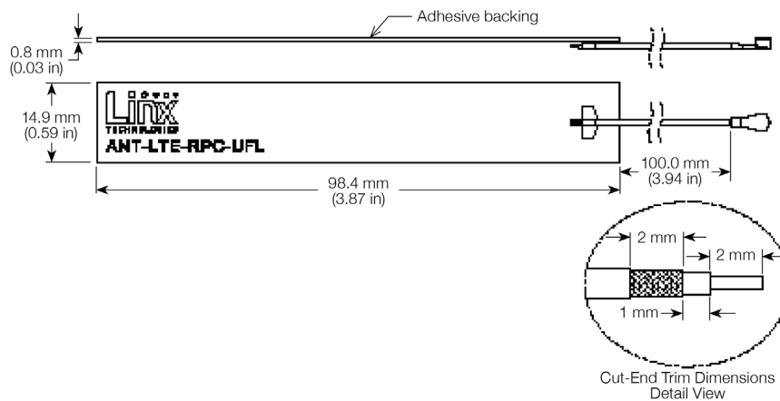
Figure 1. ANT-LTE-RPC-ccc Product Dimensions
