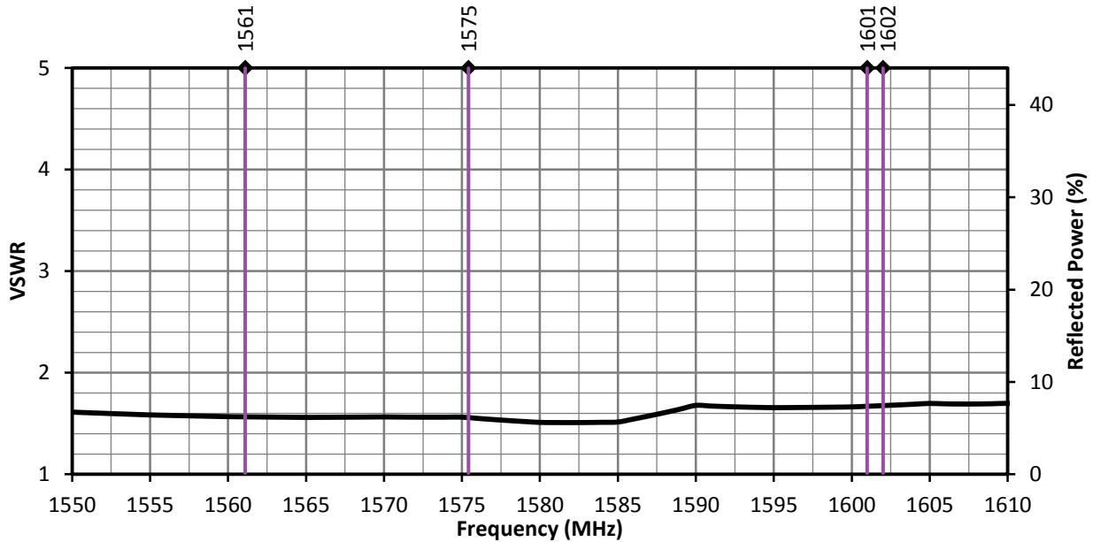
Figure 2. ANT-GNCP-C185L160 VSWR
