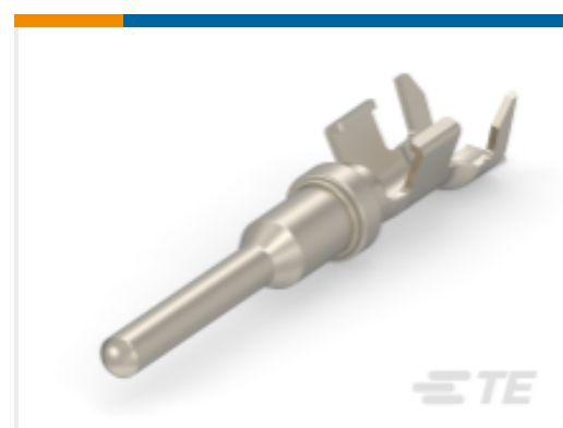
TE Part #1060-16-0122-PS PIN, SF, SIZE 16, 14-18, NI/SN, 100 PC
