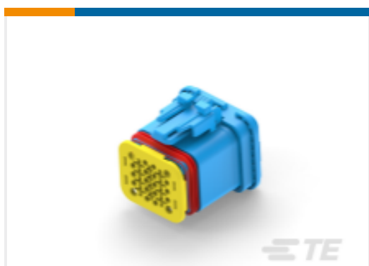
TE Part #1-2350890-4 20POS, HYBRID, SOC HSG ASSY, SLD, COD D
