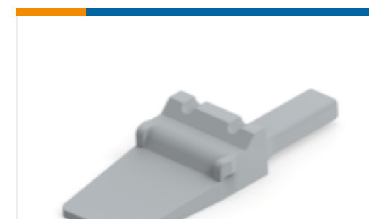
TE Part #WM-2PA WEDGE LOCK, 2P, REC, GRY, DTM, A
