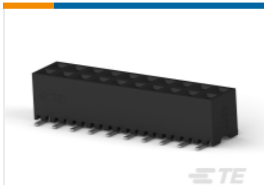
TE Part #2-2314846-0 20P,2MM,BB,REC,DRV,T,SMD,AU.76, TB,W/CP
