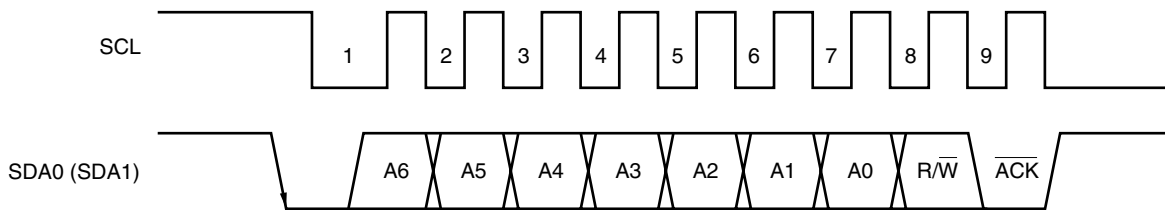
Figure 13-40. Acknowledge Signal
