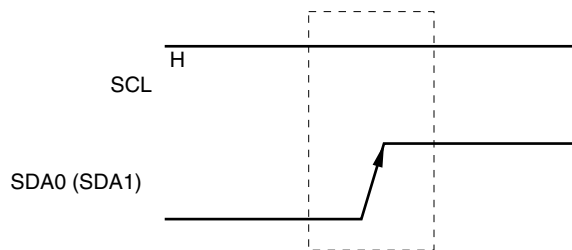
Figure 13-41. Stop Condition
