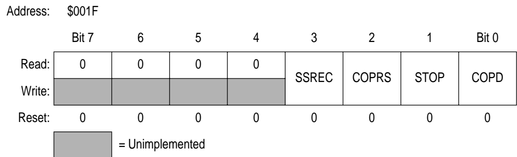
Figure 20-2. Configuration Register (CONFIG)
