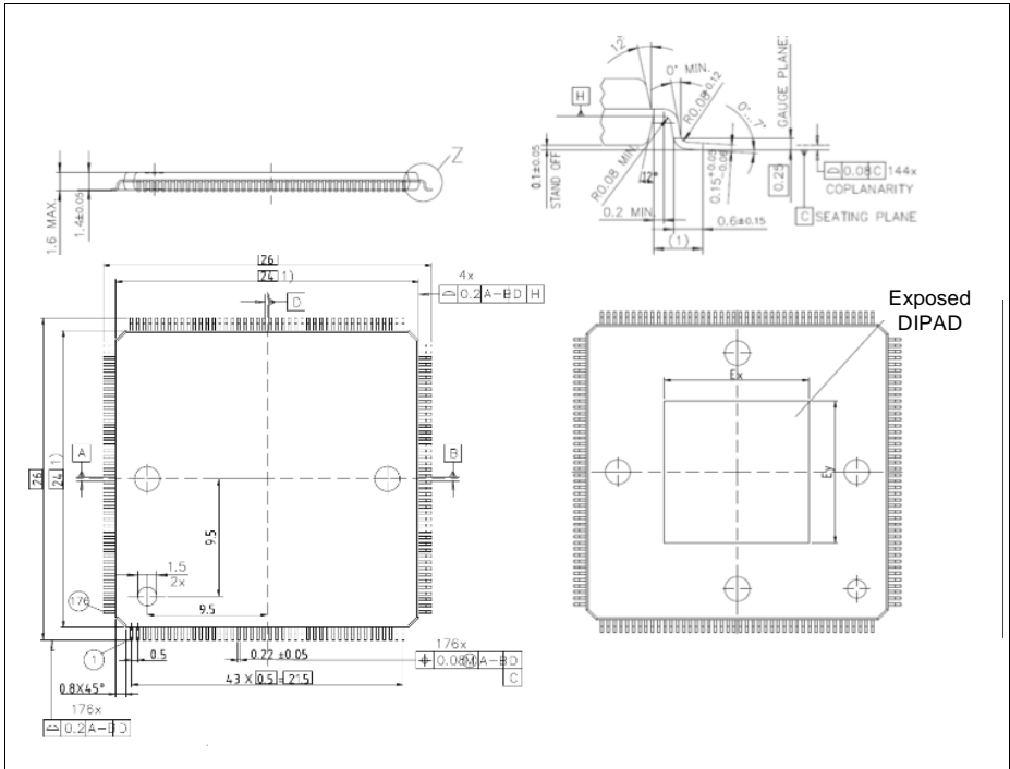
Figure 27 Package Outlines PG-LQFP-176-10
