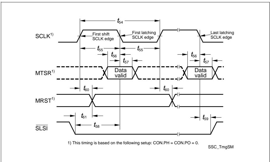
Figure 25 SSC Slave Mode Timing
