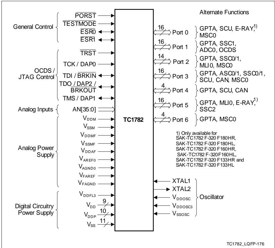
Figure 5 TC1782 Logic Symbol
