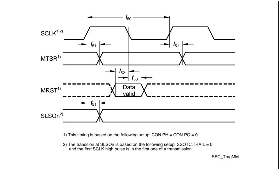
Figure 24 SSC Master Mode Timing
